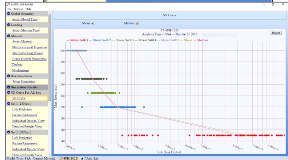
Simulated S-N Curve
